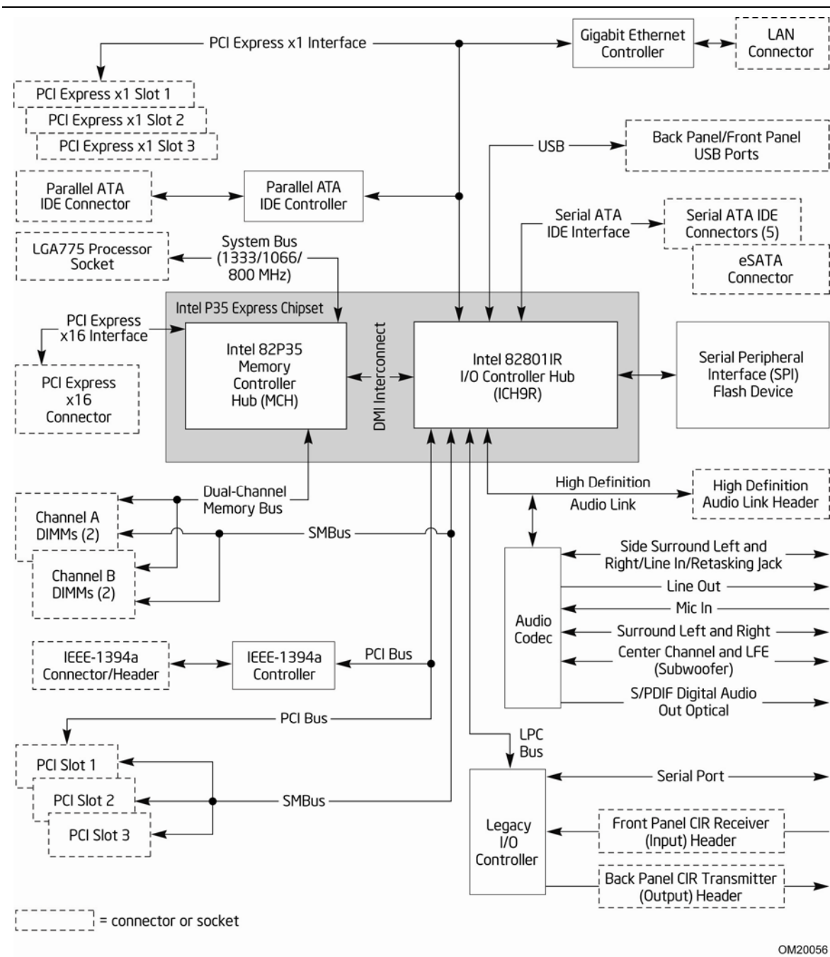
Figure 2. Block Diagram
