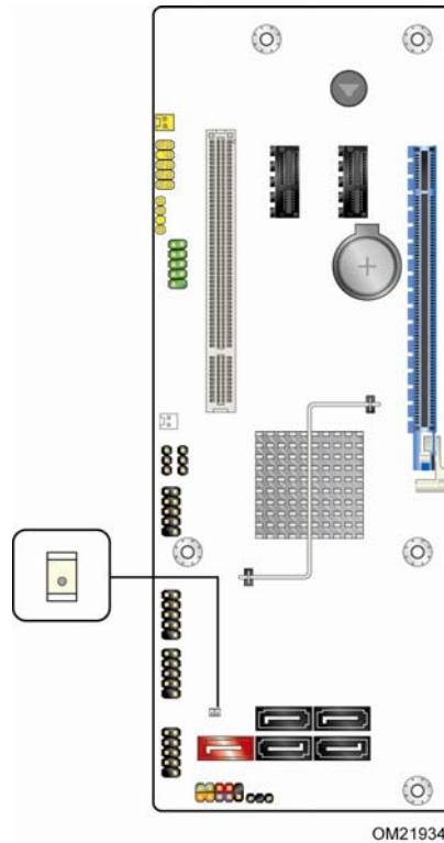
Figure 7. Location of the Intel ME "M" State LED
