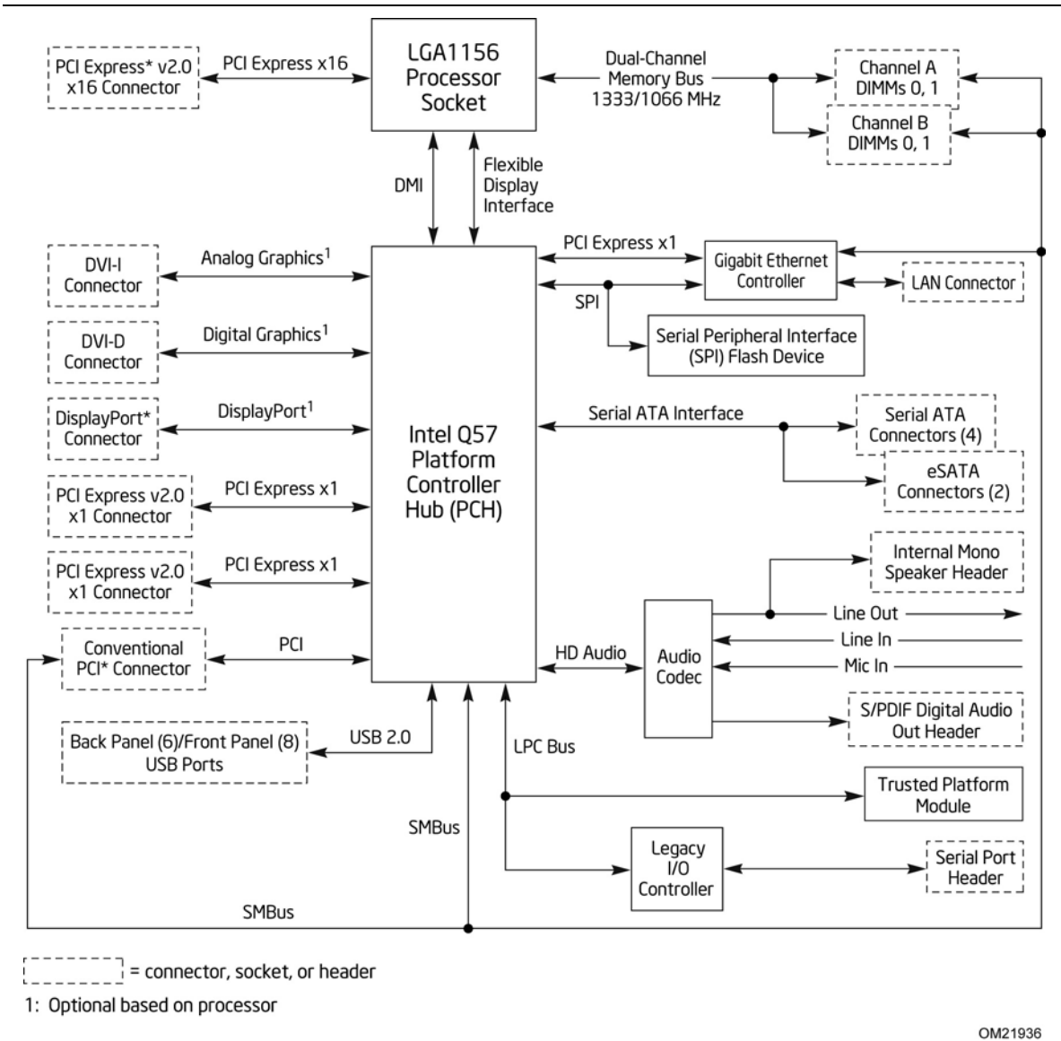
Figure 2. Block Diagram
