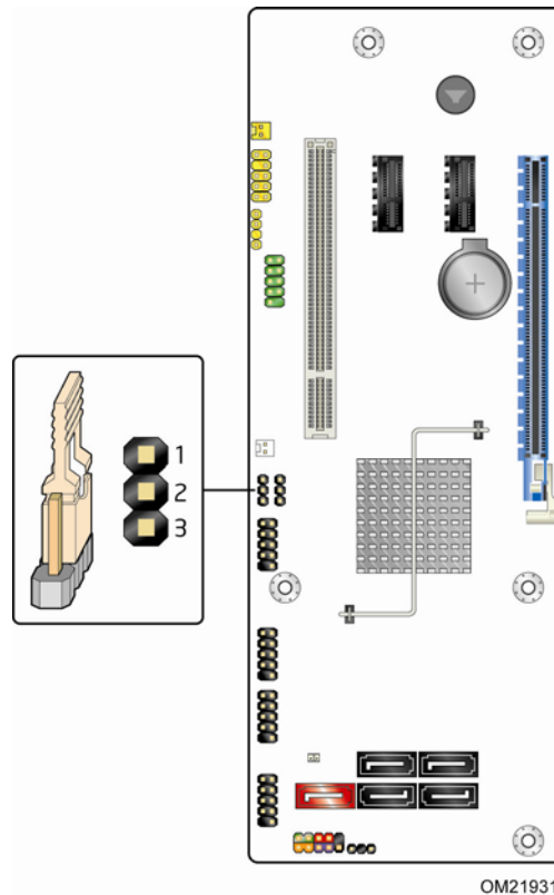
Figure 14. Location of the Jumper Block
