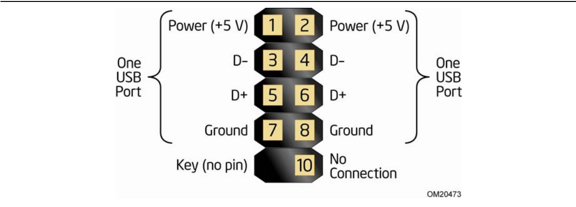
Figure 13. Connection Diagram for Front Panel USB Headers
