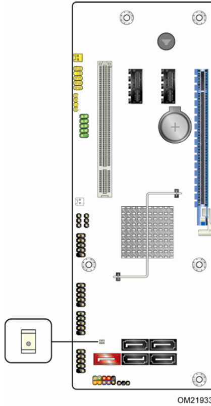
Figure 8. Location of the Standby Power LED (Green)
