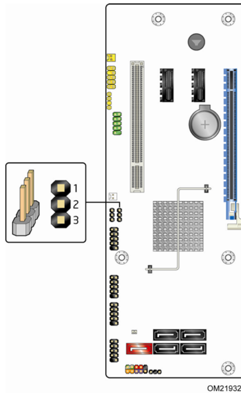
Figure 15. CMOS Clear Header
