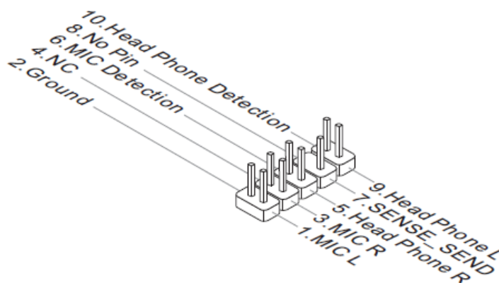
Figure 8: Front panel audio connector
