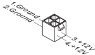
Figure 7: ATX 12V 4-PIN power connector
