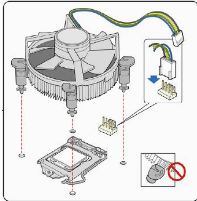
Figure 17: Connecting the processor fan heat sink power cable to the processor fan header
