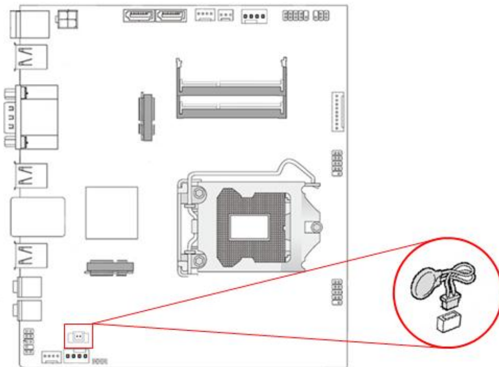
Figure 20: Removing the Battery
