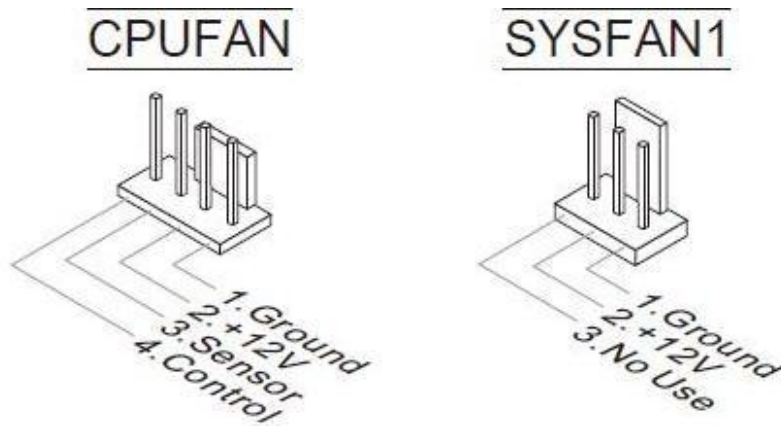
Figure 10: Fan Power connectors
