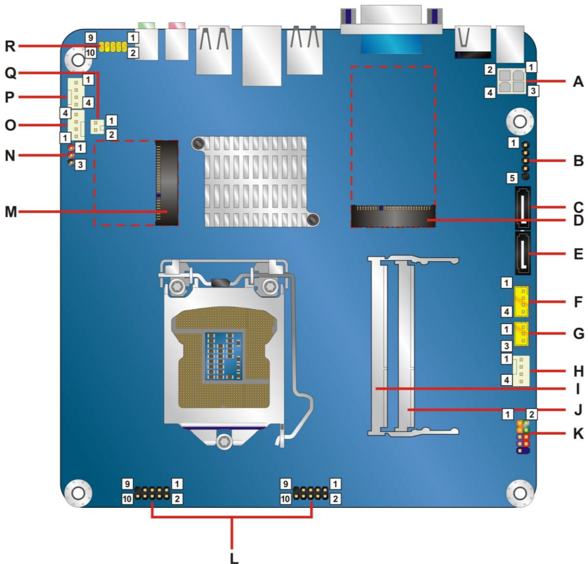
Figure 3: Motherboard Layout & Components
