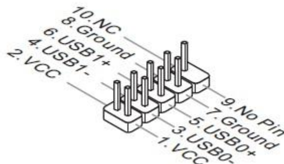
Figure 9: Front USB connectors
