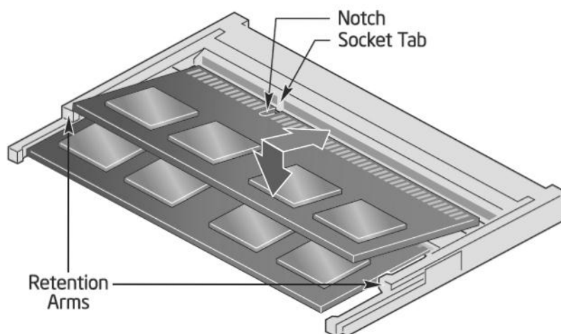
Figure 18: Memory Installation
