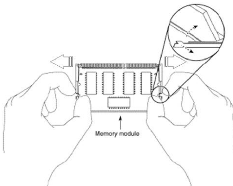
Figure 19: Removing Memory Modules
