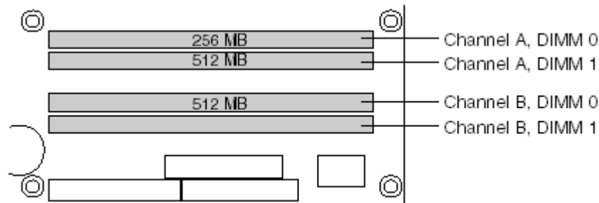
Figure 11. Single Channel (Asymmetric) Mode Configuration with Three DIMMs
