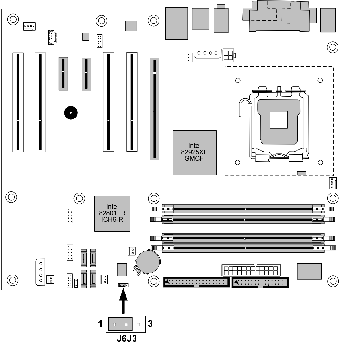
Figure 5. Motherboard jumper.
