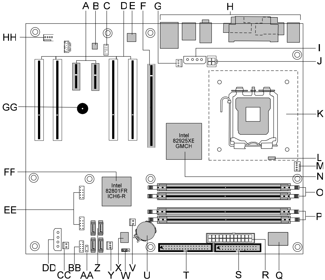
Figure 1 Motherboard Layout & Components
