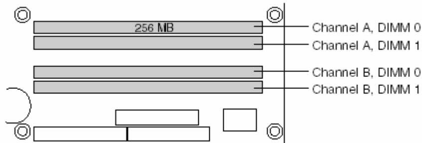
Figure 10. Single Channel (Asymmetric) Mode Configuration with One DIMM
