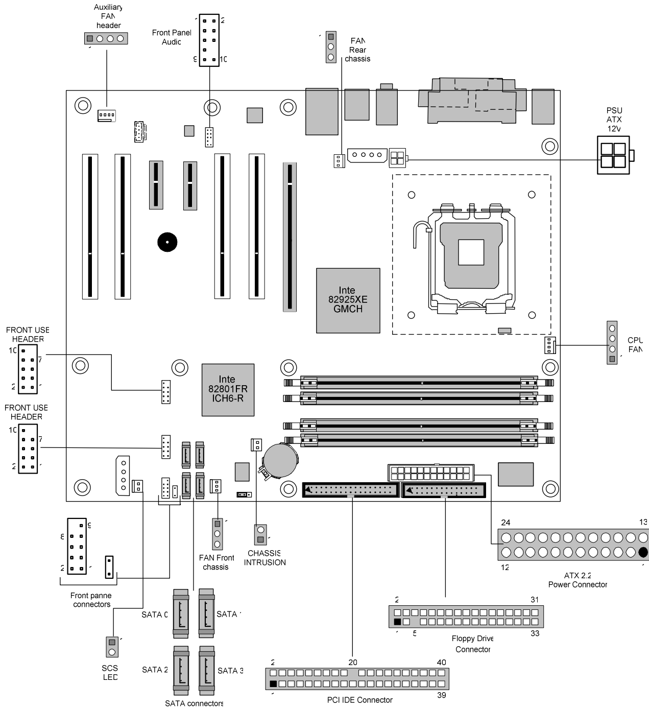
Figure 4. Motherboard Connectors
