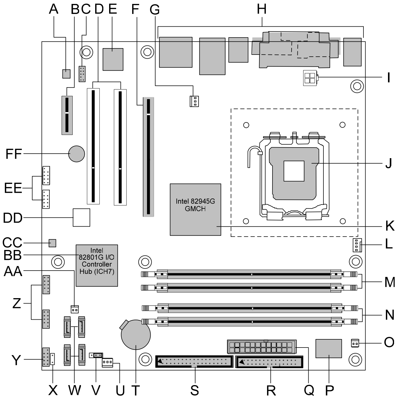
Figure 1 Motherboard Layout & Components
