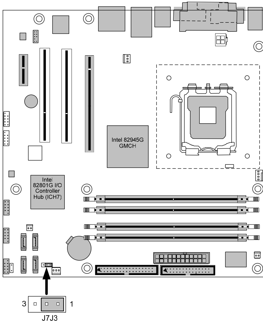
Figure 5. Motherboard jumper.
