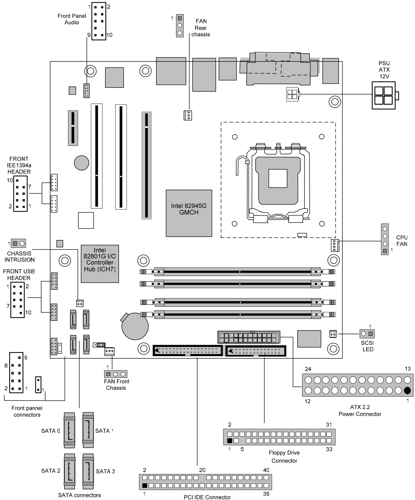
Figure 4. Motherboard Connectors
