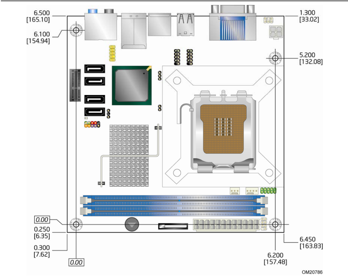
Figure 14. Board Dimensions
