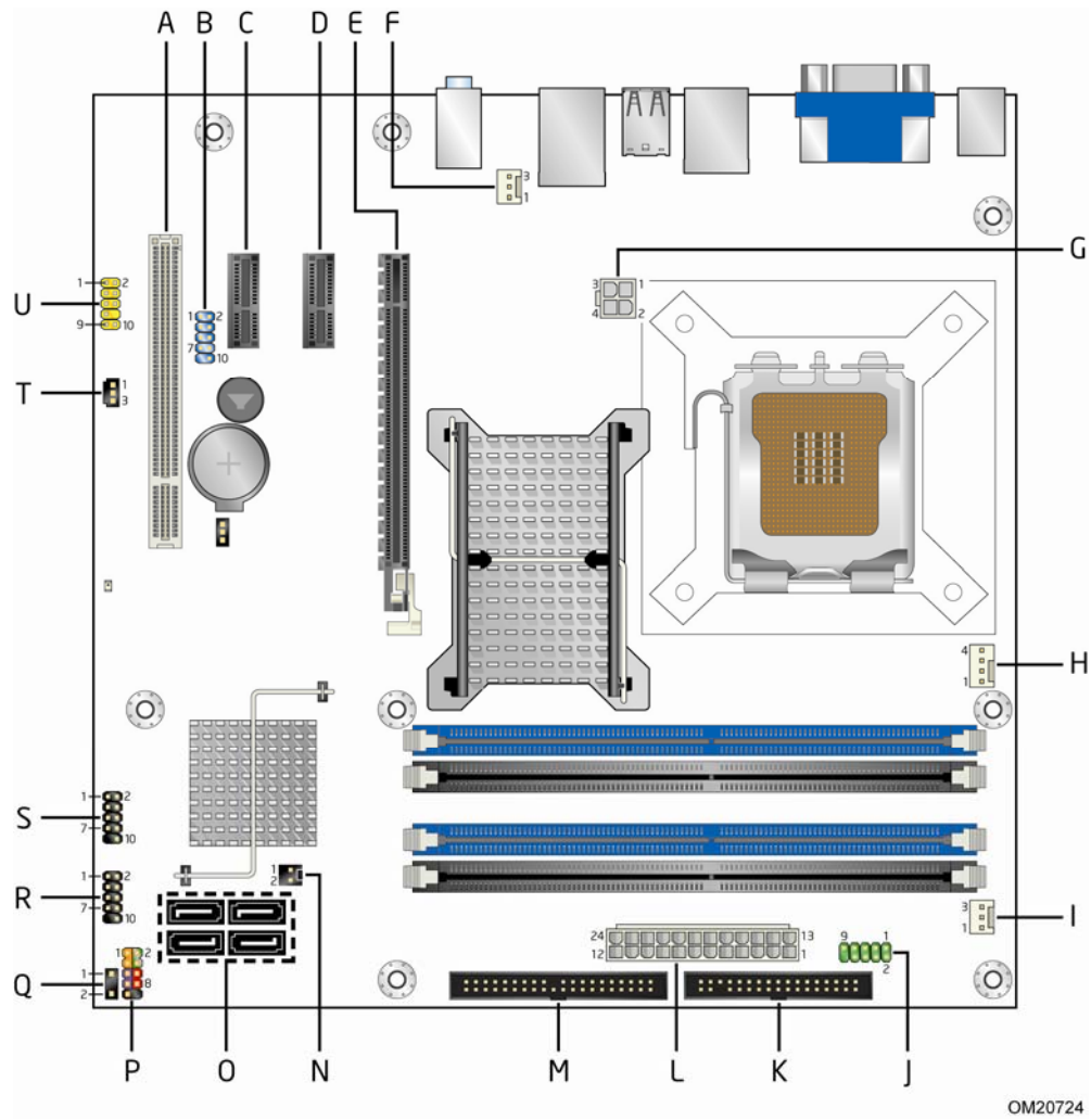
Figure 10. Component-side Connectors and Headers
