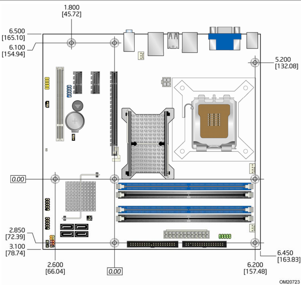
Figure 14. Board Dimensions
