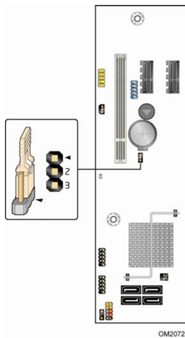
Figure 13. Location of the Jumper Block
