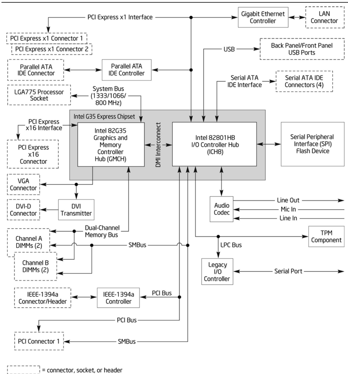
Figure 2. Block Diagram
