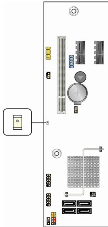
Figure 7. Location of the Standby Power Indicator LED
