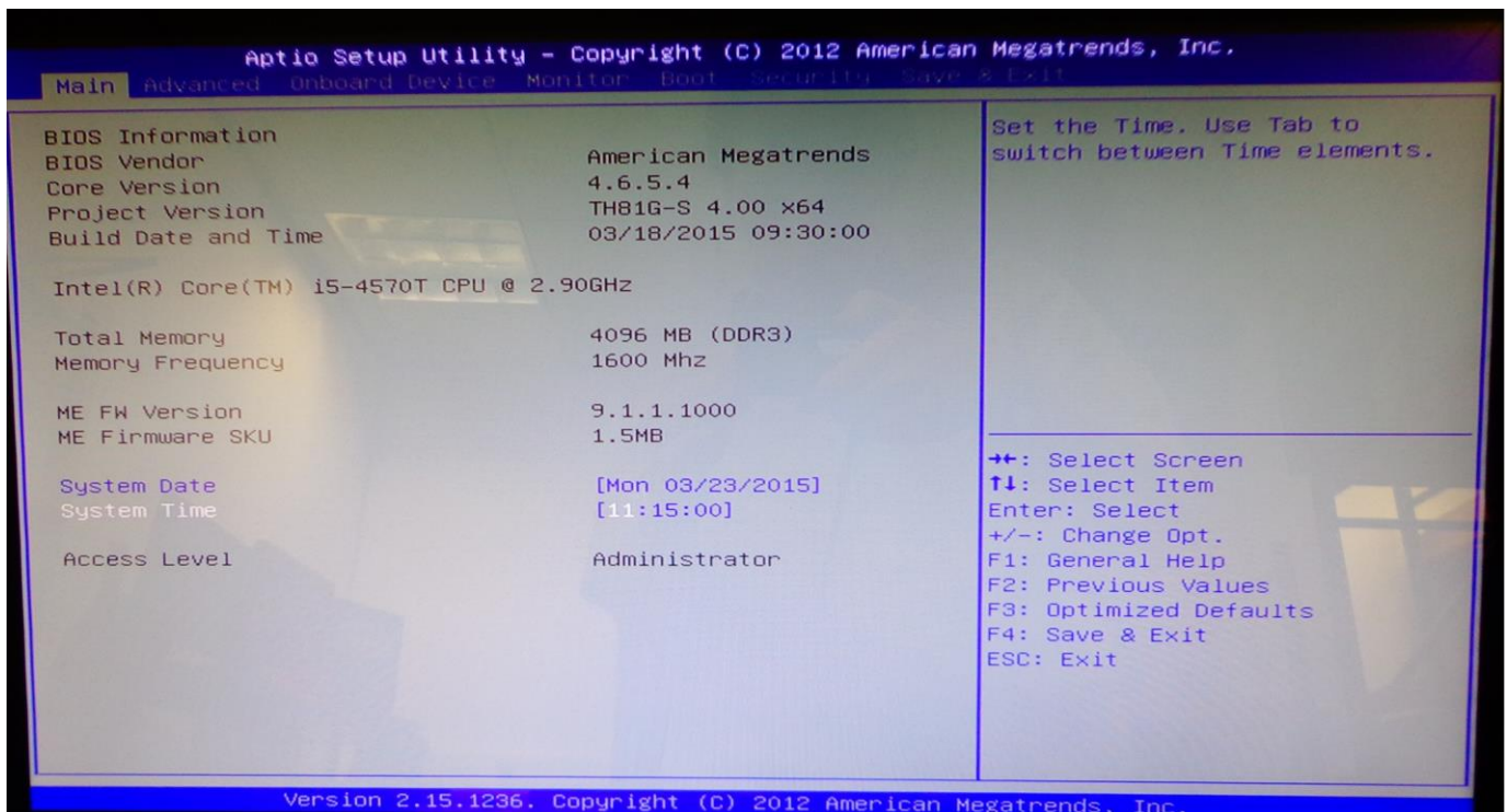
Figure 22: Main Menu
