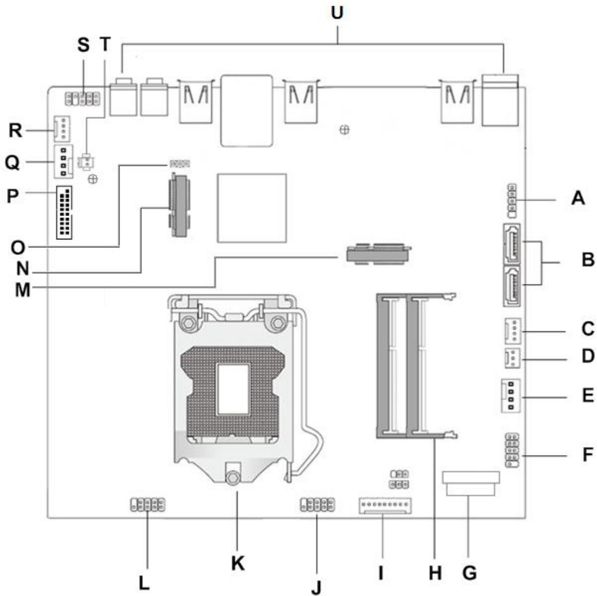
Figure 3: Motherboard Layout
