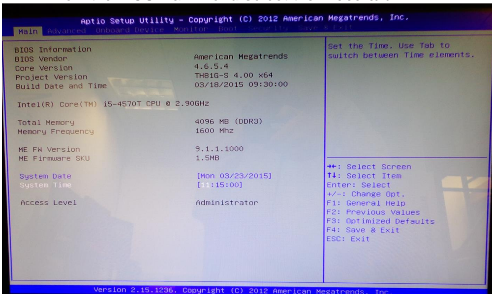
Figure 26: Main menu
