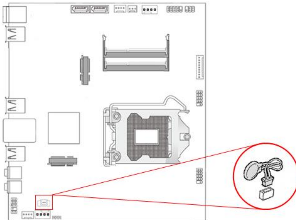
Figure 21: Removing the Battery
